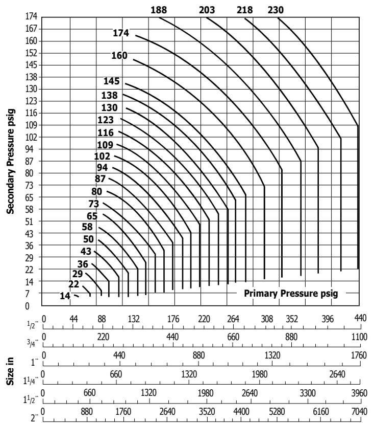
→ Steam Flow lb/h
